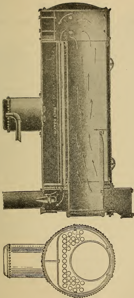
FIG. 30.—SECTIONAL VIEWS OF THE NEW GIANT BOILER.
